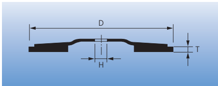
Flat (Type 27)
