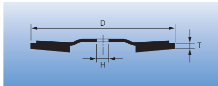
Conical (Type 29)
